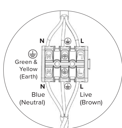
Connector Block Detail
