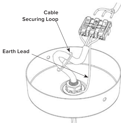
Ceiling Rose Internal View
