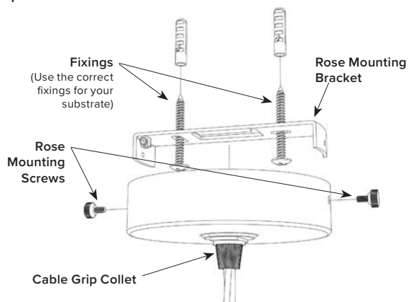
Ceiling Rose Mounting
