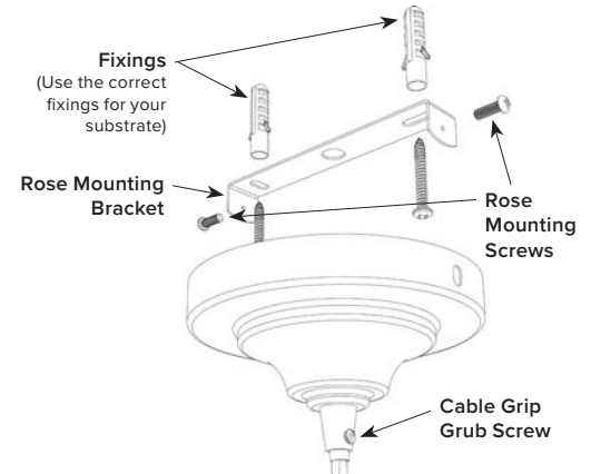
Ceiling Rose Mounting
